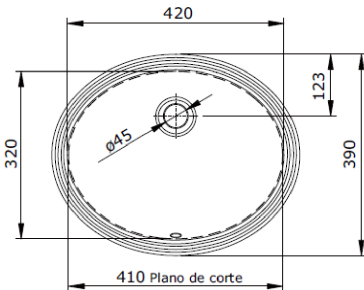
Sanindusa — Simple Under Counter Basin Model No.— 108750
